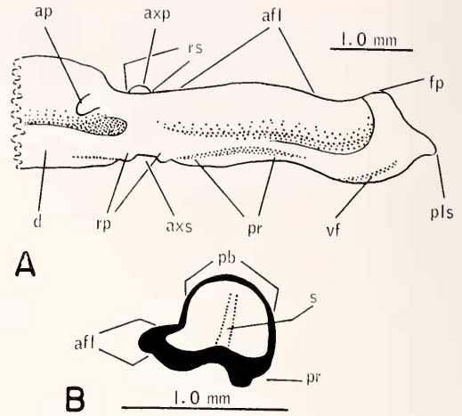
Figure 8. Fragiscutum rhythium n. gen., n. sp. A) Ventral view of part of a segment. Compare Plate 12, figures 13, 14, 17, 20. B) Section through inner part of pleura, in exsagittal plane. Solid block is replaced outer portion of exoskeleton. Abbreviations: afl, anterior flange; ap, apodeme; axp, axial articulating process; axs, axial articulating socket; d, doublure of axial ring; fp, projection at anterior margin of facet; pb, pleural band; pls, pleural spine; pr, posterior recess; rp, ring articulating process; rs, ring articulating socket; s, silicified lining of conal, appearing as a hollow cone (compare Pl. 13, fig. 17); vf, vincular furrow.
